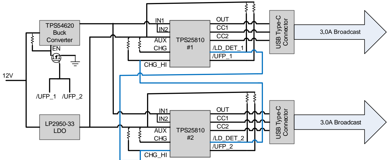
Figure 16. PPM and Power Wake Implemented
