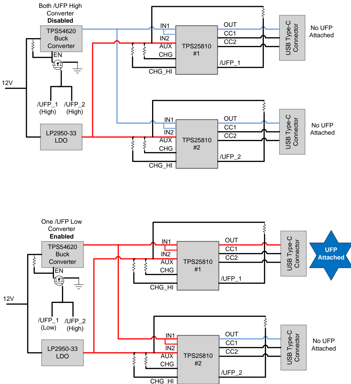
Figure 15. Power Wake Implementation
