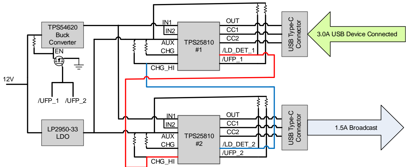
Figure 17. 3-A USB Device Connected
