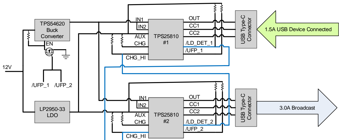
Figure 18. 1.5-A USB Device Connected
